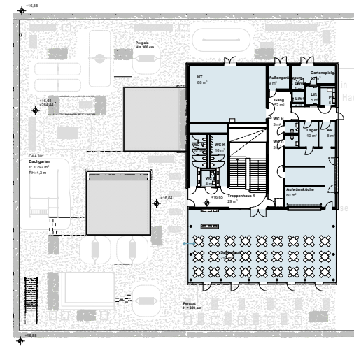
4. Obergeschoss fourth floor
